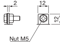
Terminal 3 Bolt and nut type M5
