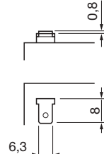
Terminal 2 Faston
