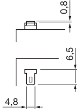
Terminal 1 Faston
