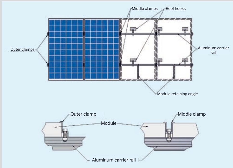
Construction of pitched roof mounting system
